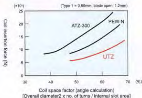
Coil insertion force during the insertion test
