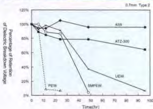
Changes in Insulation Performance due to Hydrolysis
